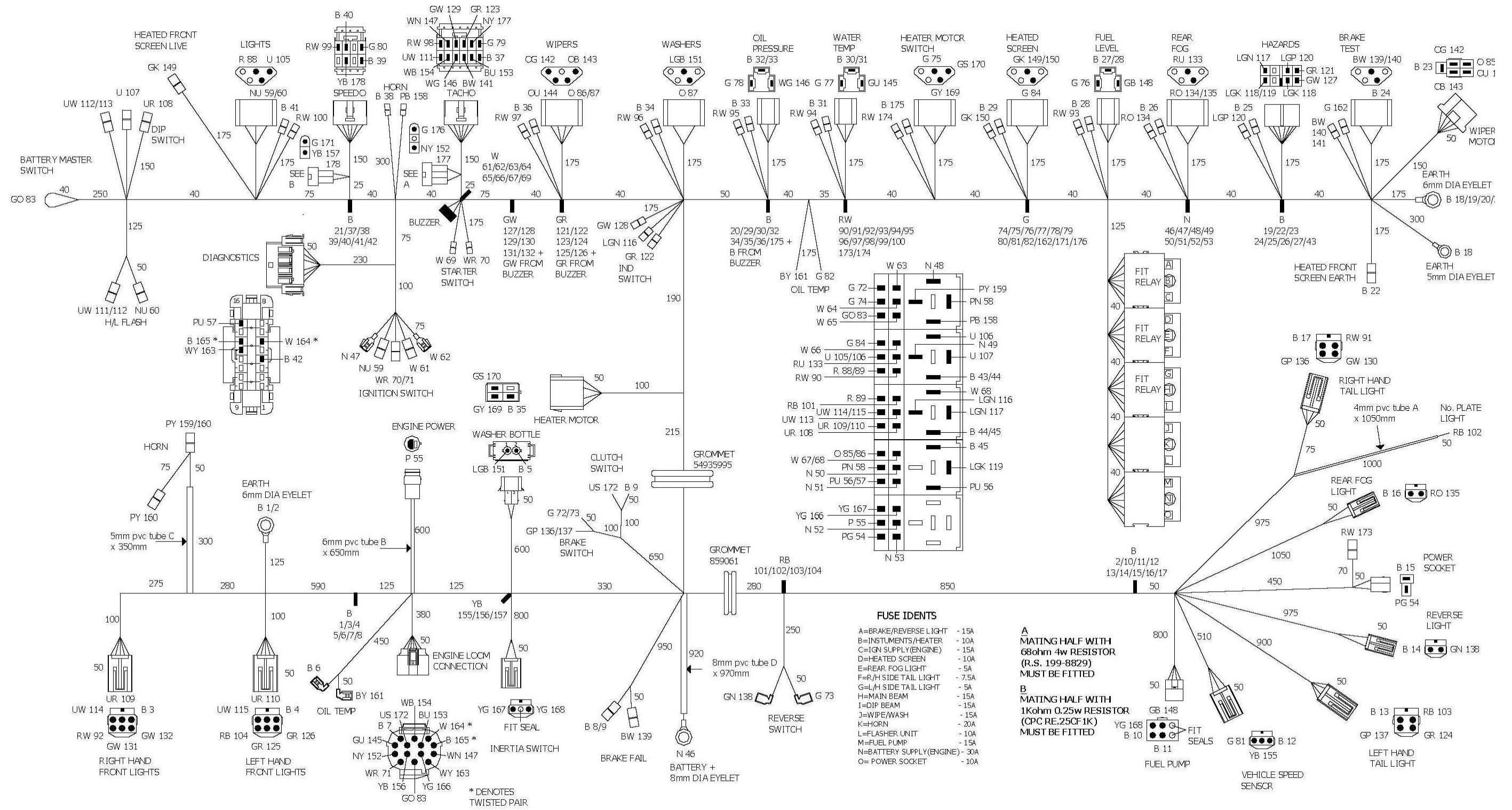
Figure 218: R400 main chassis harness (standard dash)
