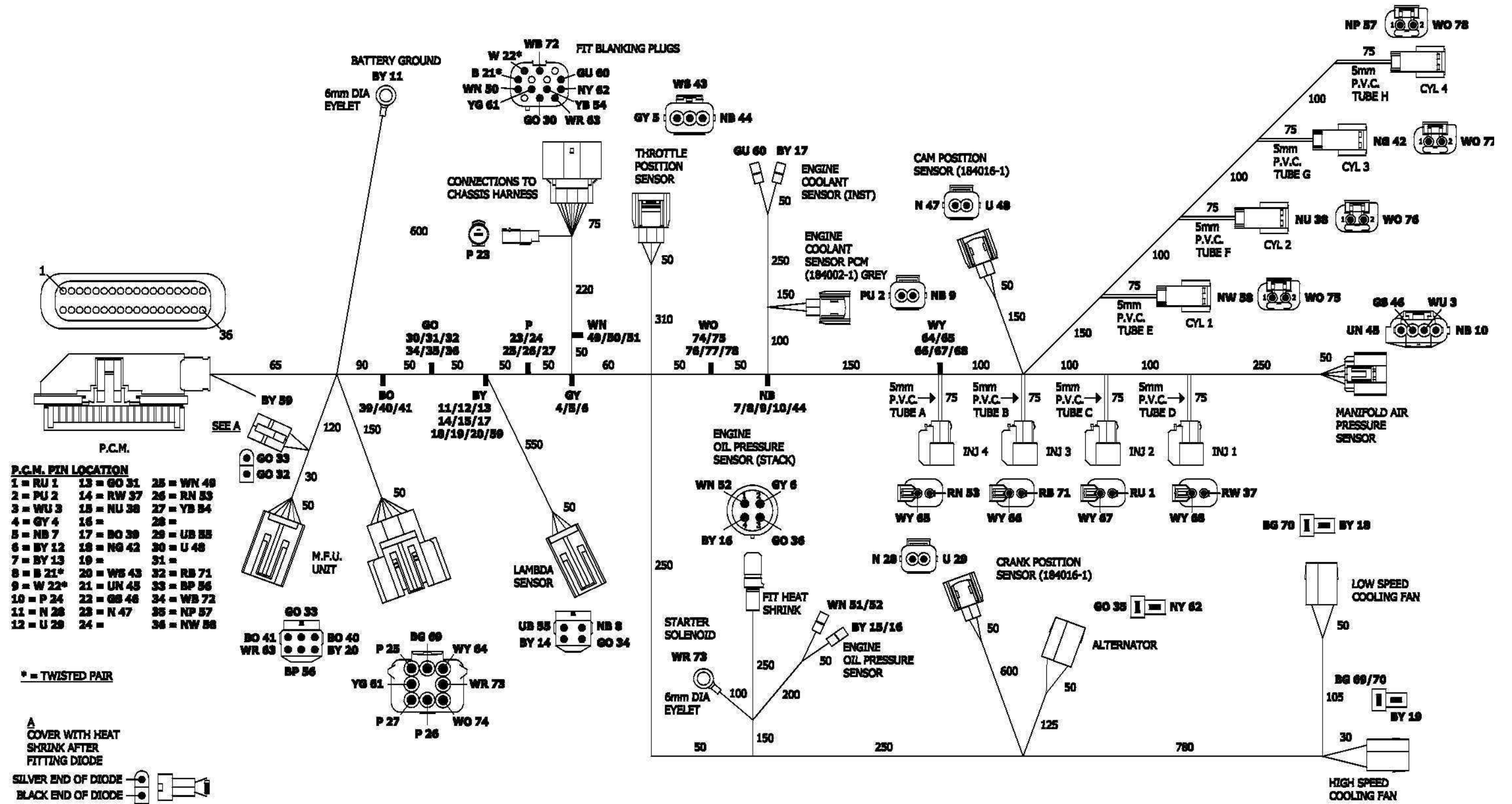
Figure 217: R400 engine harness
